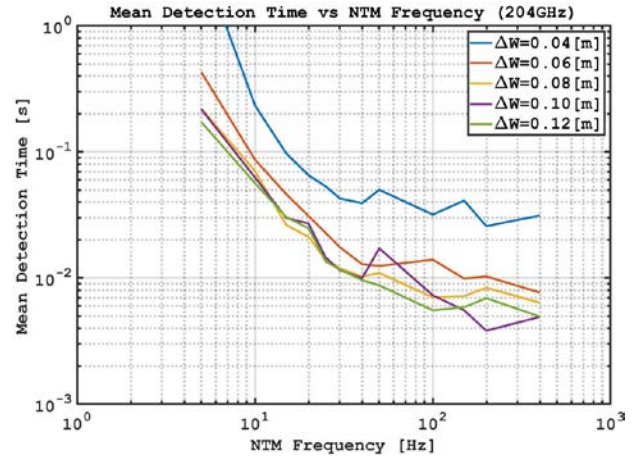
Fig. 4: Mean mode detection time simulated for different mode size and rotation frequencies.
