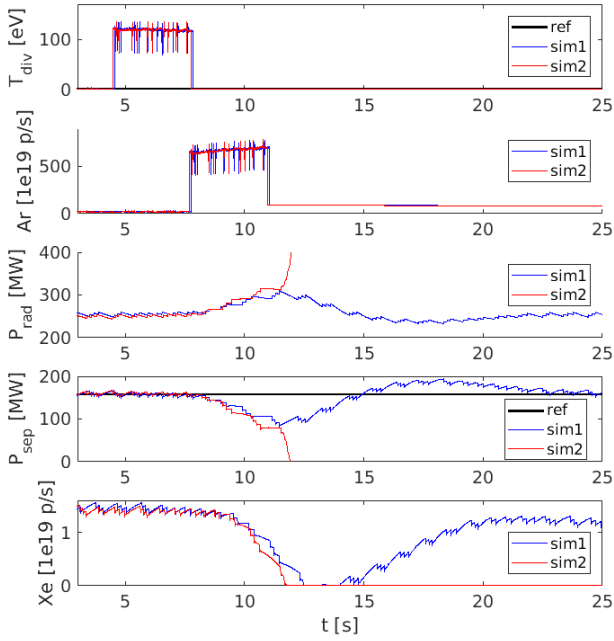
Fig. 3: Simulation of divertor detachment control after prescribed reattachment: sim1 with assumed argon enrichment factor 20; sim2 with enrichment factor 15 [73].
