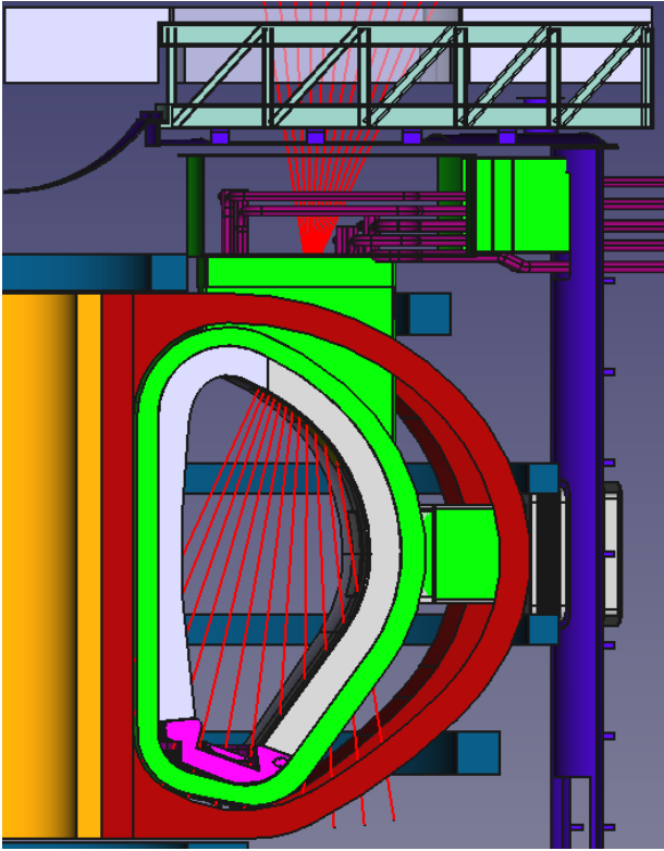
Fig. 8: Poloidal cross section with vertical lines of sight of the neutron diagnostics
